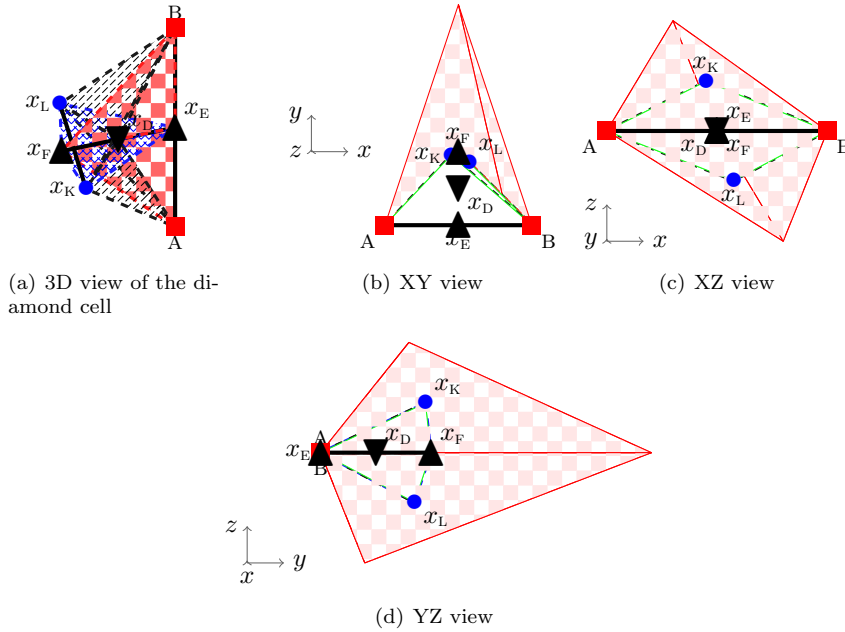
FIGURE 2.2. Example mesh with tetrahedrons.
