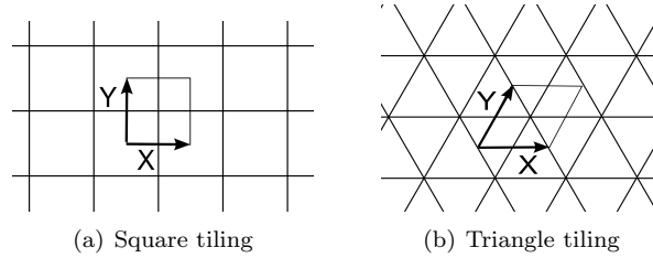
Figure 2. FVT actions of the group p1 .
