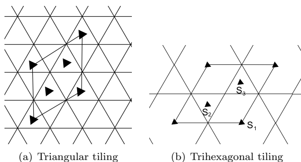
Figure 14. FVT actions of the group p3 .
