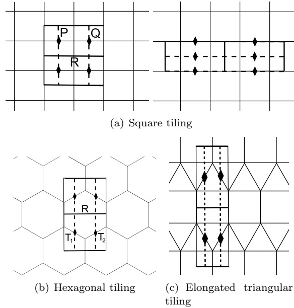
Figure 9. FVT actions of the group pmg .
