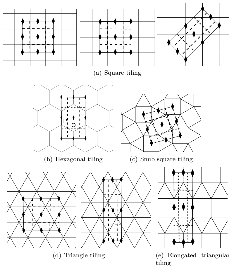
Figure 10. FVT actions of the group pgg .
