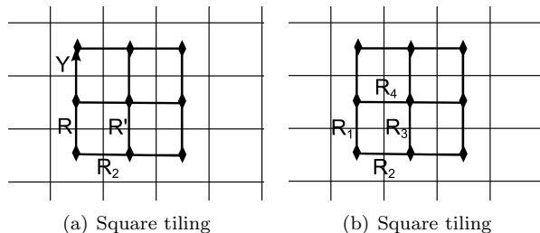
Figure 7. FVT actions of the group pmm .
