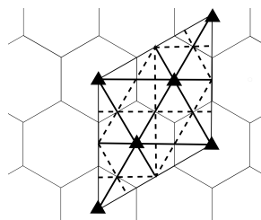
Figure 17. An FVT action of the group p3m1 .
