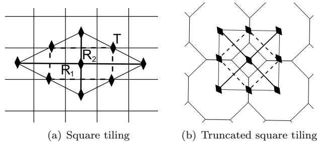
Figure 12. FVT actions of the group cmm .
