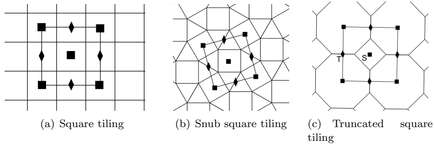
Figure 6. FVT actions of the group p4 .
