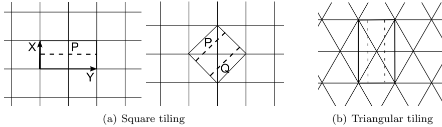
Figure 5. FVT actions of the group pg .
