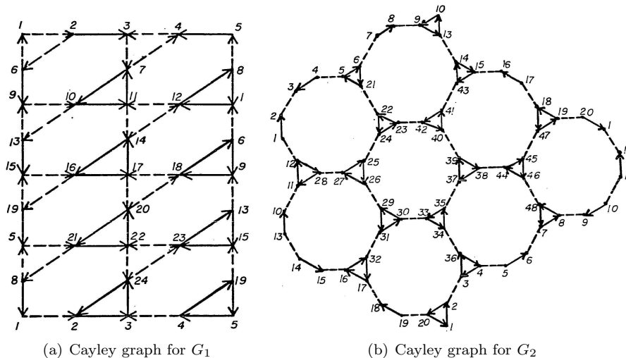
Figure 19. Proulx toroidal Cayley graphs.
