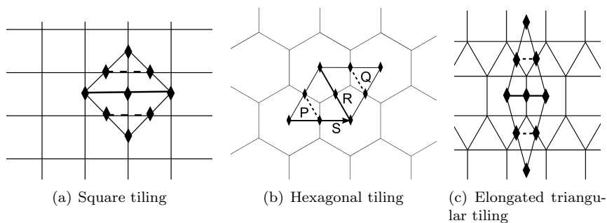
Figure 8. FVT actions of the group cm .
