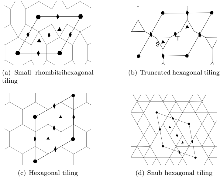
Figure 15. FVT actions of the group p6 .
