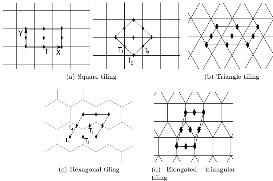
Figure 3. FVT actions of the group p2 .
