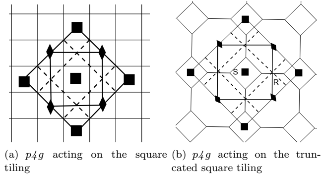
Figure 11. FVT actions of the group p4g .
