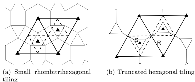
Figure 16. FVT actions of the group p31m .
