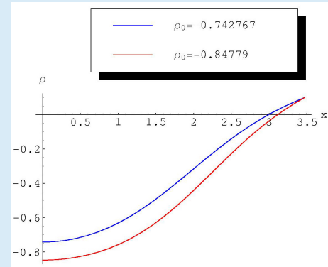
FIG. 4.1. \lambda = 1 , c(x) = 1 and \xi = 0.1
