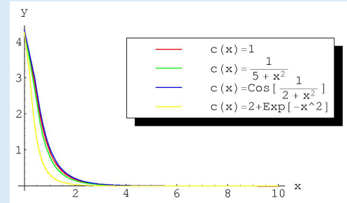
(b) Solutions of the problem (1.1)–(1.3)
