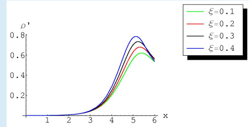
FIG. 4.2. Graphics of solutions and their derivatives in the case N = 3 , M = 6 and c(x) = \sin\left(1 + \frac{1}{1+x^2}\right)
