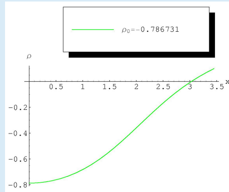
FIG. 4.1. \lambda = 1 , c(x) = 1 and \xi = 0.1
