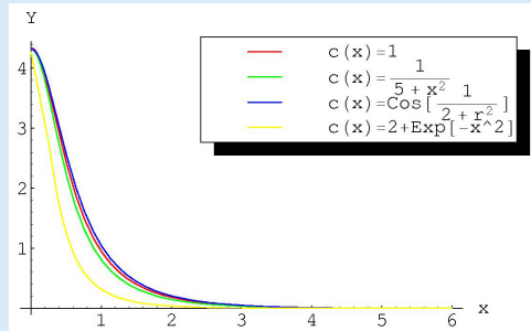
(a) Solutions of the problem (1.1)–(1.2) with M = 6
