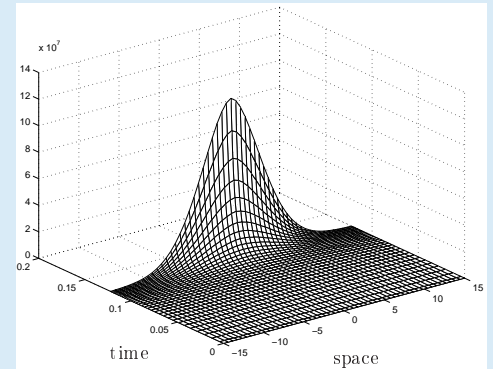
FIG. 6.4. Evolution of the numerical solution ( q = p , L > L_1 )
