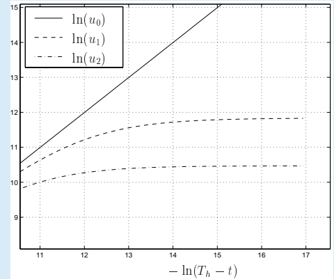
FIG. 6.6. If 3 = q > p = 2.3 the blow-up set consist on K = 2 nodes
