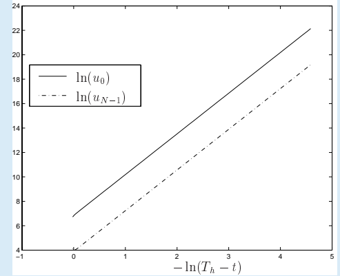
FIG. 6.2. Blow-up rates ( q = p )
