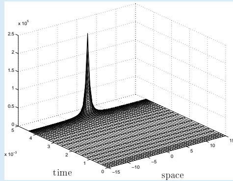
FIG. 6.5. Evolution of the numerical solution ( q > p )
